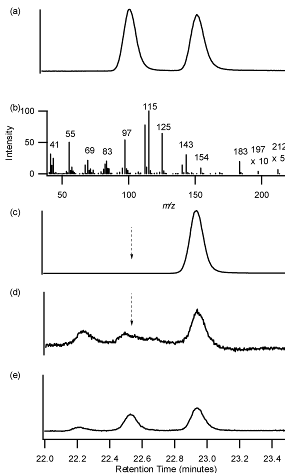
Fig. 6 Total ion current (TIC) of enantioselective GC traces employing single ion monitoring of m/z 212, 183, 143, 125, and 112. (a) Racemic ( E,E )- 1 . (b) Mass spectrum of synthetic 1 . (c) Enantiomerically pure ( 2S,6R,8S )- 1 . (d) Concentrated pentane extract of female B. tryoni abdomens. (e) Co-injection of concentrated extract with racemic ( E,E )- 1 .
